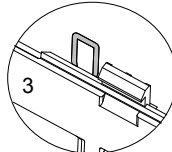
图 7-8 MD310T0.4B、MD310T0.7B、MD310T1.5B、MD310T2.2B、MD310T3.7B、MD310T5.5B 安规电容跳线位置及断开方法
