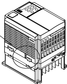
图 7-8 MD310T0.4B、MD310T0.7B、MD310T1.5B、MD310T2.2B、MD310T3.7B、MD310T5.5B 安规电容跳线位置及断开方法
